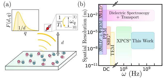
FIG. 1. (a) Schematic of qubit sensing experiment. A probe qubit (top right), with splitting \omega_q , is a distance d away from a polar or dielectric material. Fluctuations in the material’s dipoles lead to electrical noise at the location of qubit causing the qubit to relax from |1\rangle to |0\rangle at a rate 1/T_1 . The qubit is sensitive to fluctuations at frequency \omega_q and wavevectors around 1/d (see filter on top left). (b) Regimes of applicability of qubit sensors and other probes including microscopy techniques [atomic-force, piezoresponse-force, and transmission electron microscopy (AFM, PFM, and TEM)], spectroscopy techniques [x-ray photon correlation, x-ray linear dichroism, and second harmonic generation spectroscopy (XPCS, XRLD, and SHG)] and electrical transport techniques [10–16, 49]. Techniques that often require high intensity light sources are marked with a *.
